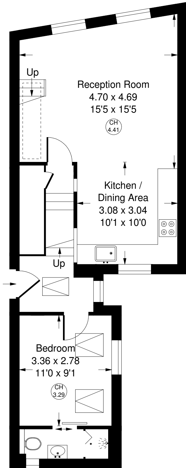
Second Floor
